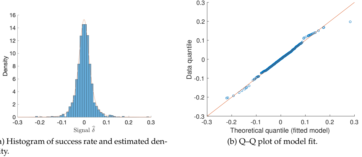
Figure 3: Model fit
